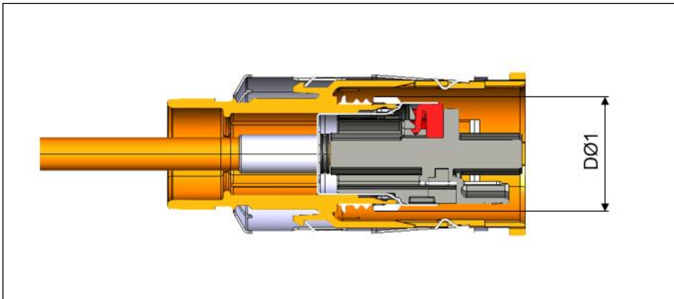
Figure 5.5: Representation 4.0 mm 2 & 6.0 mm 2 SCC dimension D\emptyset1 (5.1 Assembling the locking sleeve)
